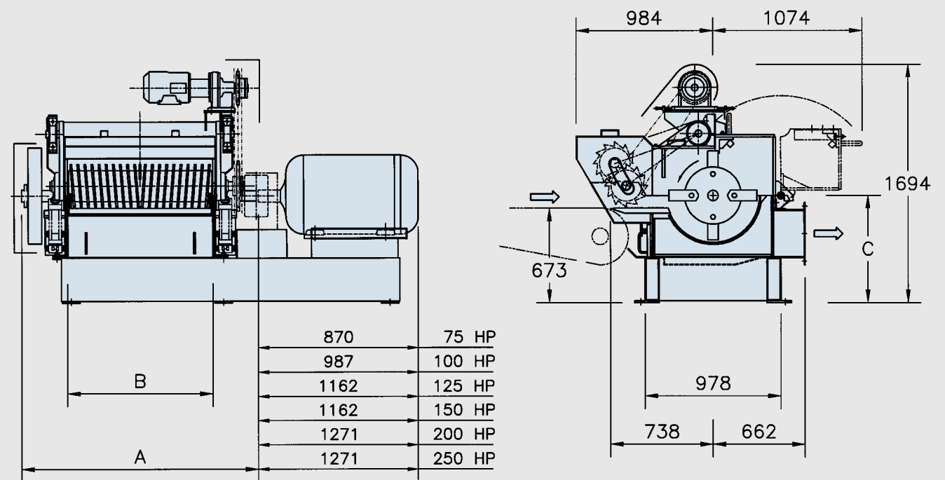
HORIZONTAL INFEED WITH HOLD DOWN ROLL MOTORIZED
